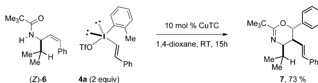
Scheme 4. Diastereoselectivity in the Cu-catalyzed oxyvinilation.
